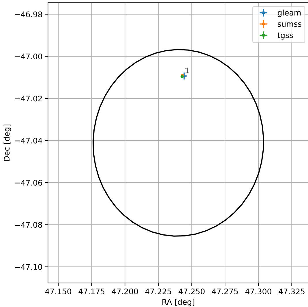
4FGL J0308.9-4702
