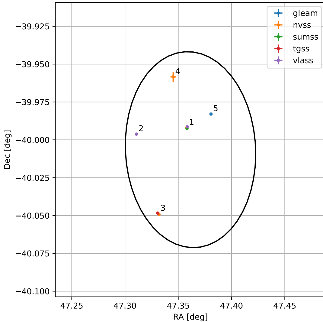
4FGL J0309.4-4000
