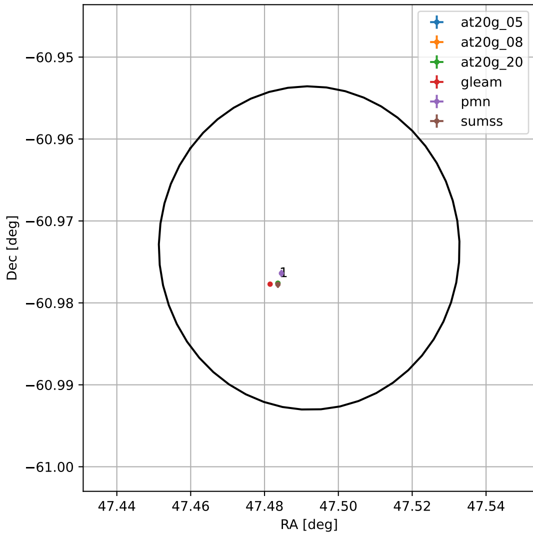
4FGL J0309.9-6058
