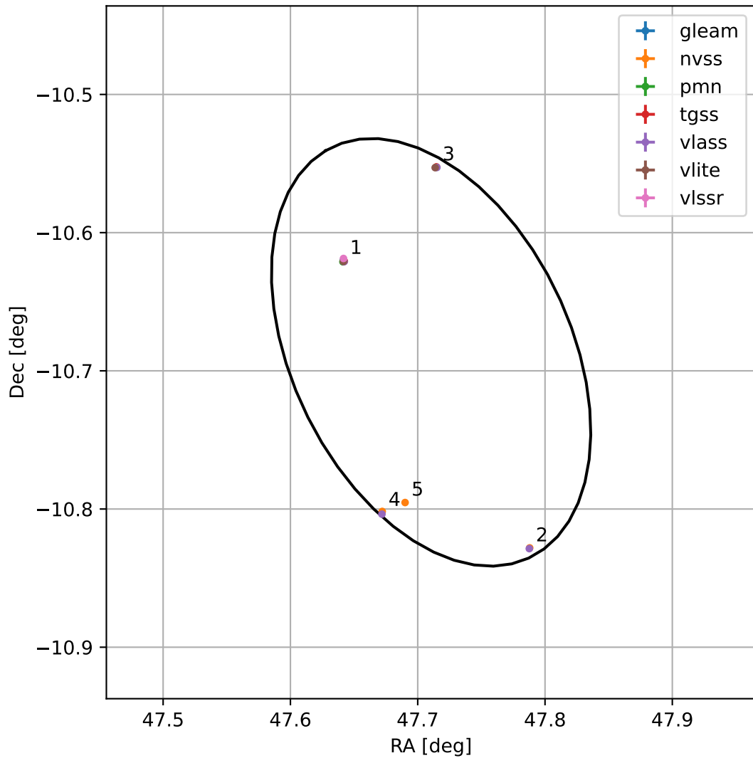
4FGL J0310.8-1041
