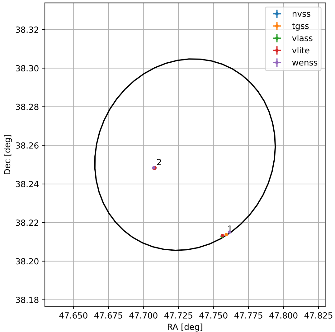
4FGL J0310.9+3815
