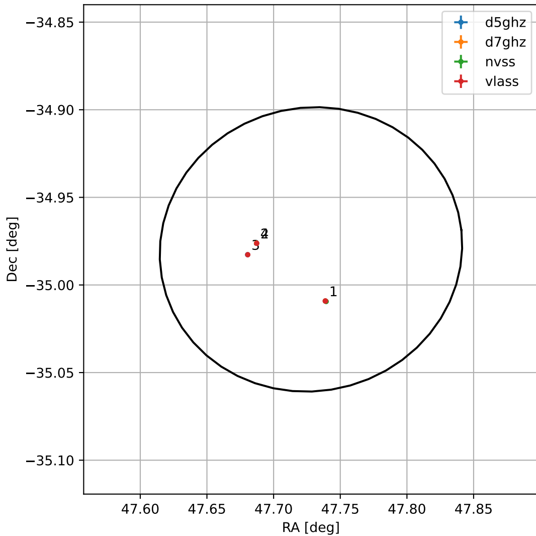
4FGL J0310.9-3458
