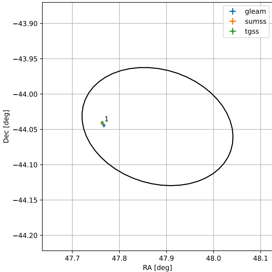
4FGL J0311.5-4402
