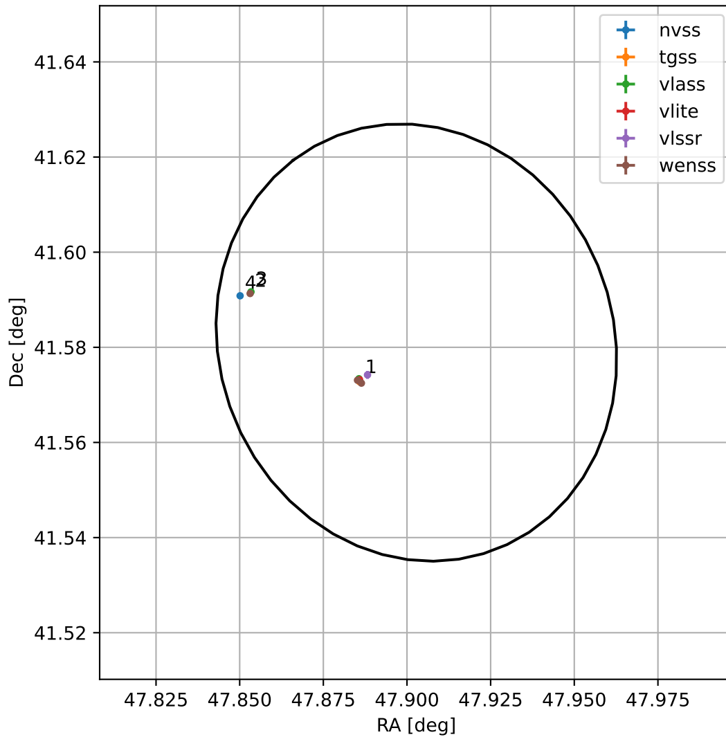
4FGL J0311.6+4134
