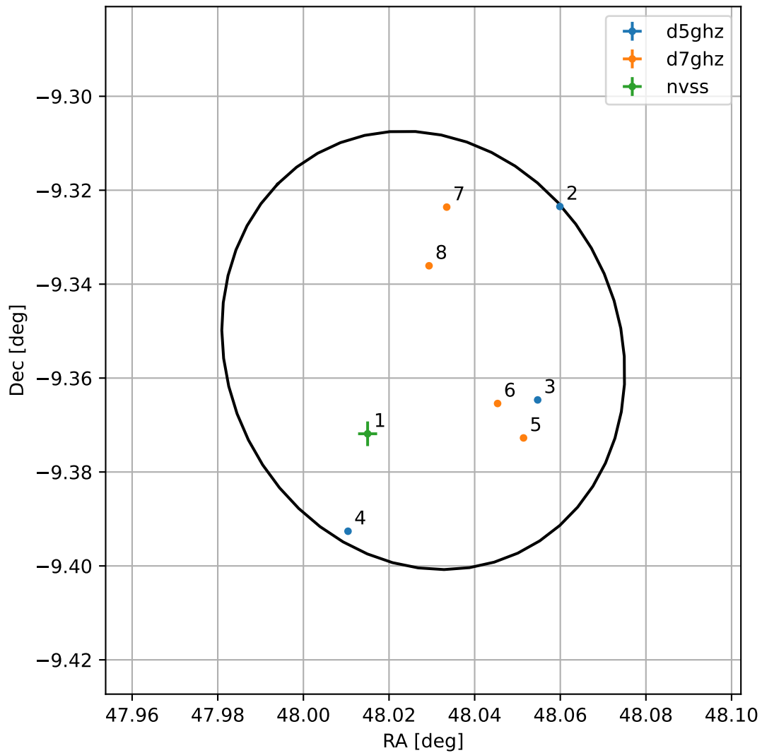
4FGL J0312.1-0921
