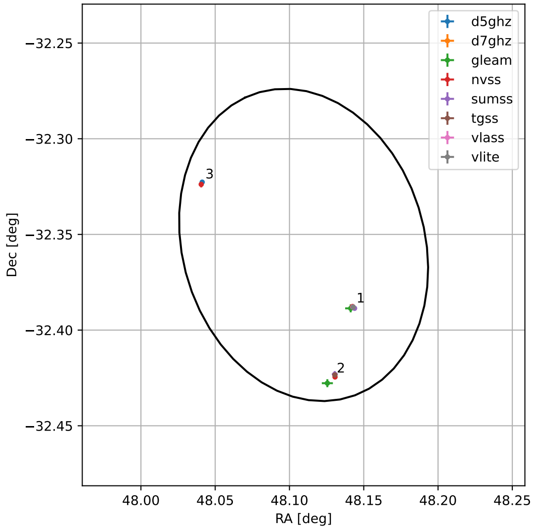
4FGL J0312.4-3221
