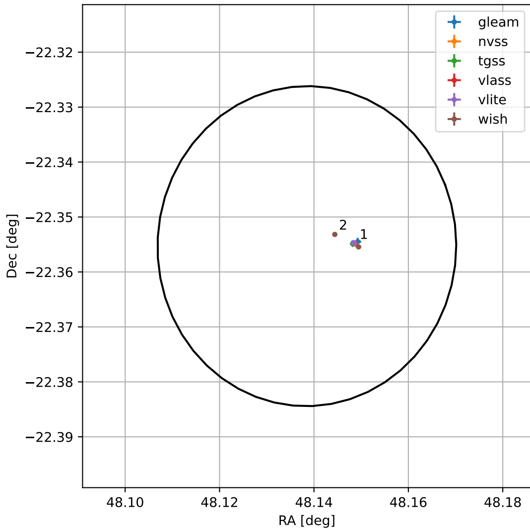
4FGL J0312.5-2221
