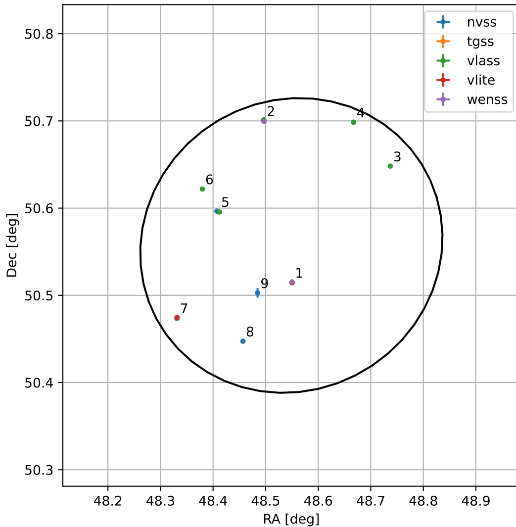
4FGL J0314.1+5033
