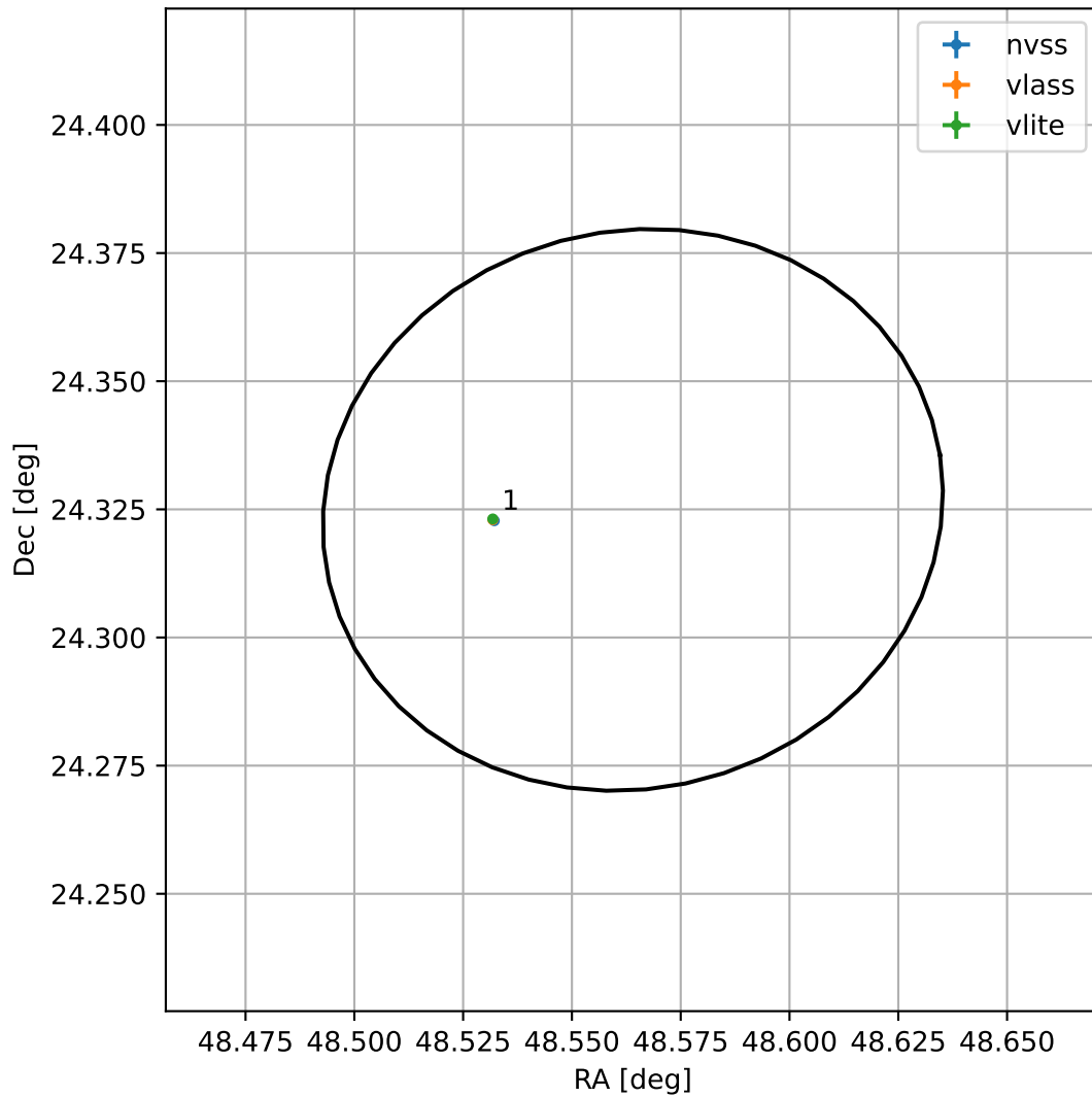
4FGL J0314.2+2419
