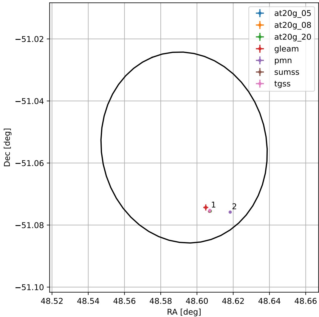
4FGL J0314.3-5103
