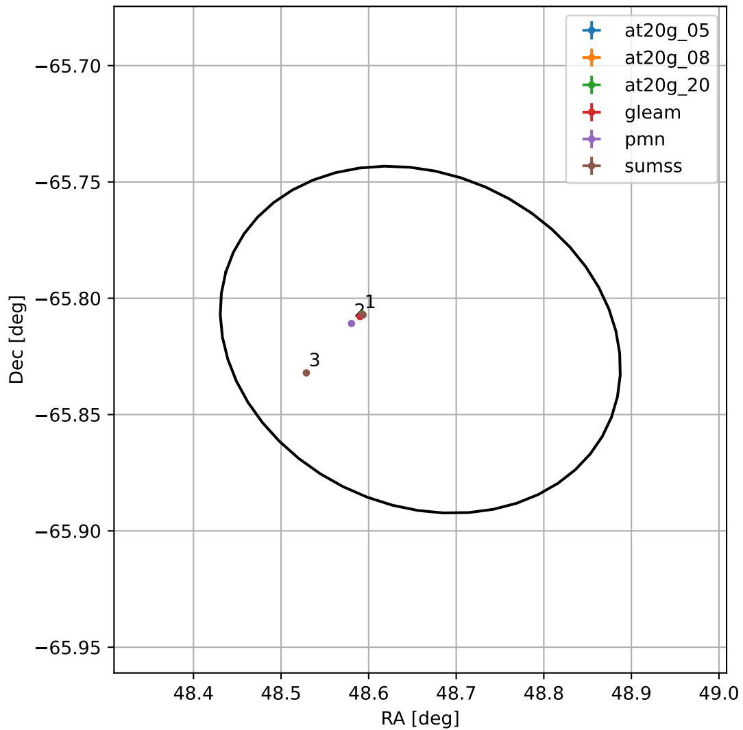
4FGL J0314.6-6549
