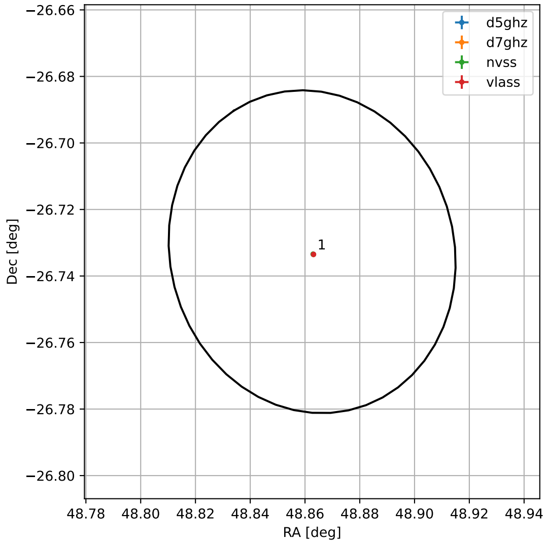
4FGL J0315.4-2643
