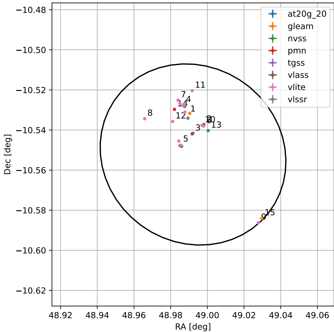
4FGL J0315.9-1033
