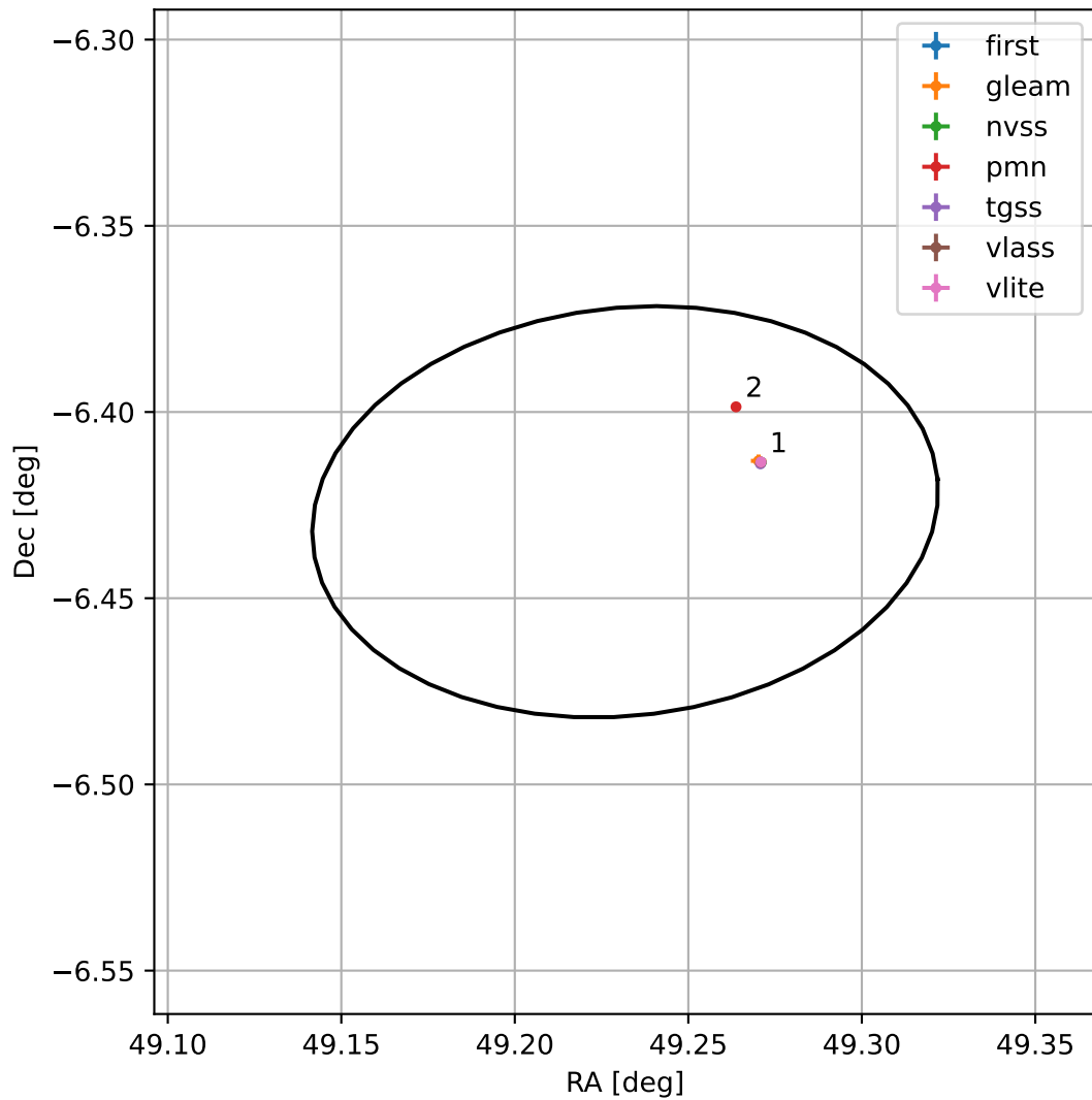
4FGL J0316.9-0625
