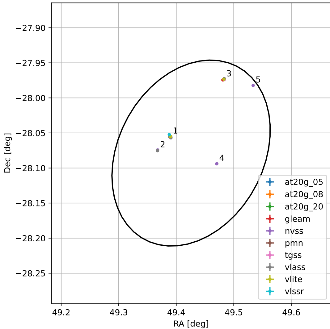
4FGL J0317.7-2804
