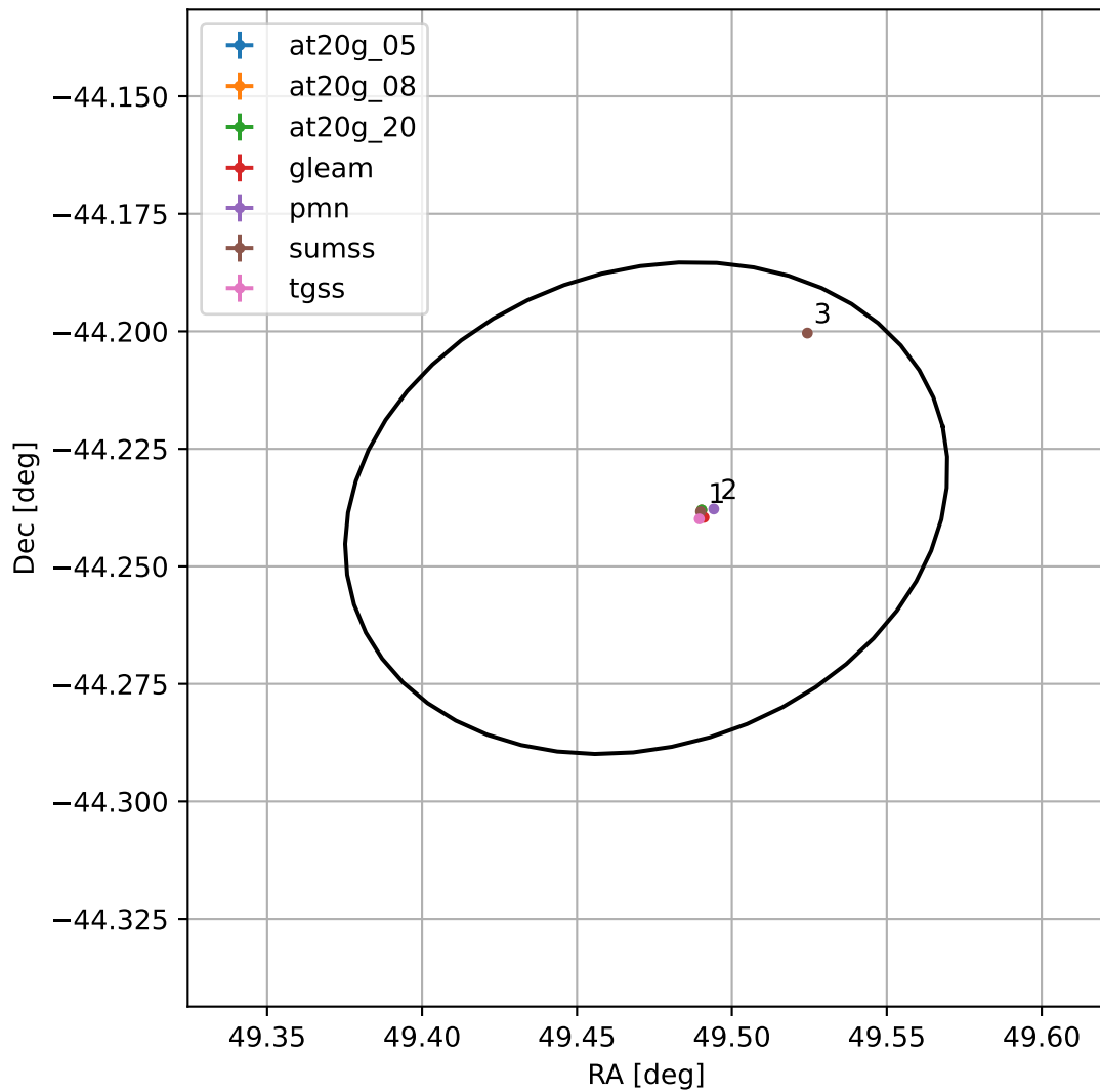
4FGL J0317.8-4414
