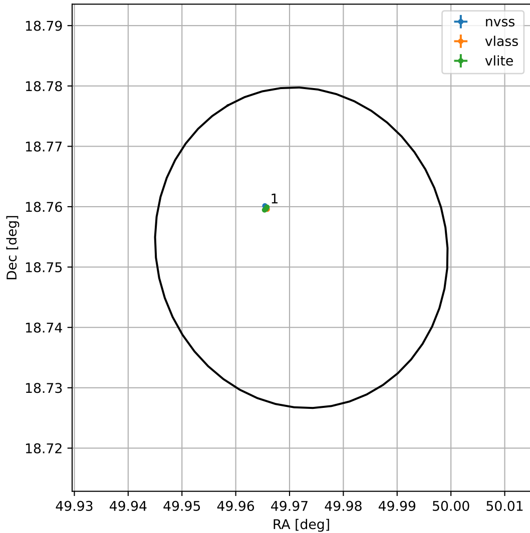
4FGL J0319.8+1845
