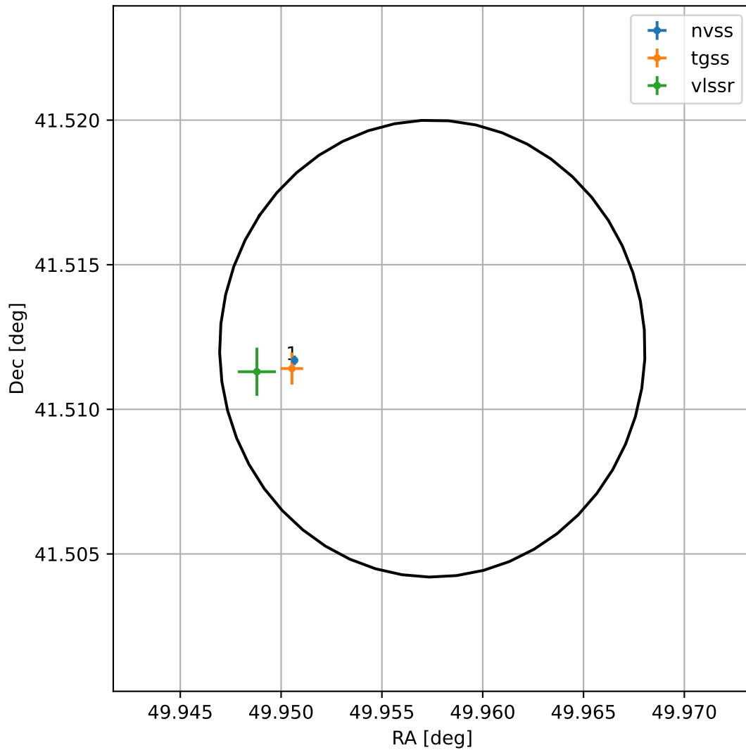
4FGL J0319.8+4130
