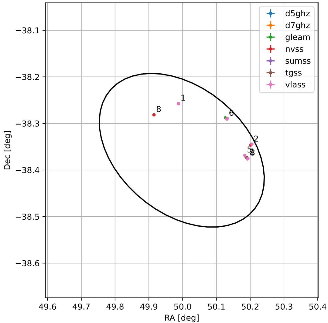
4FGL J0319.9-3821
