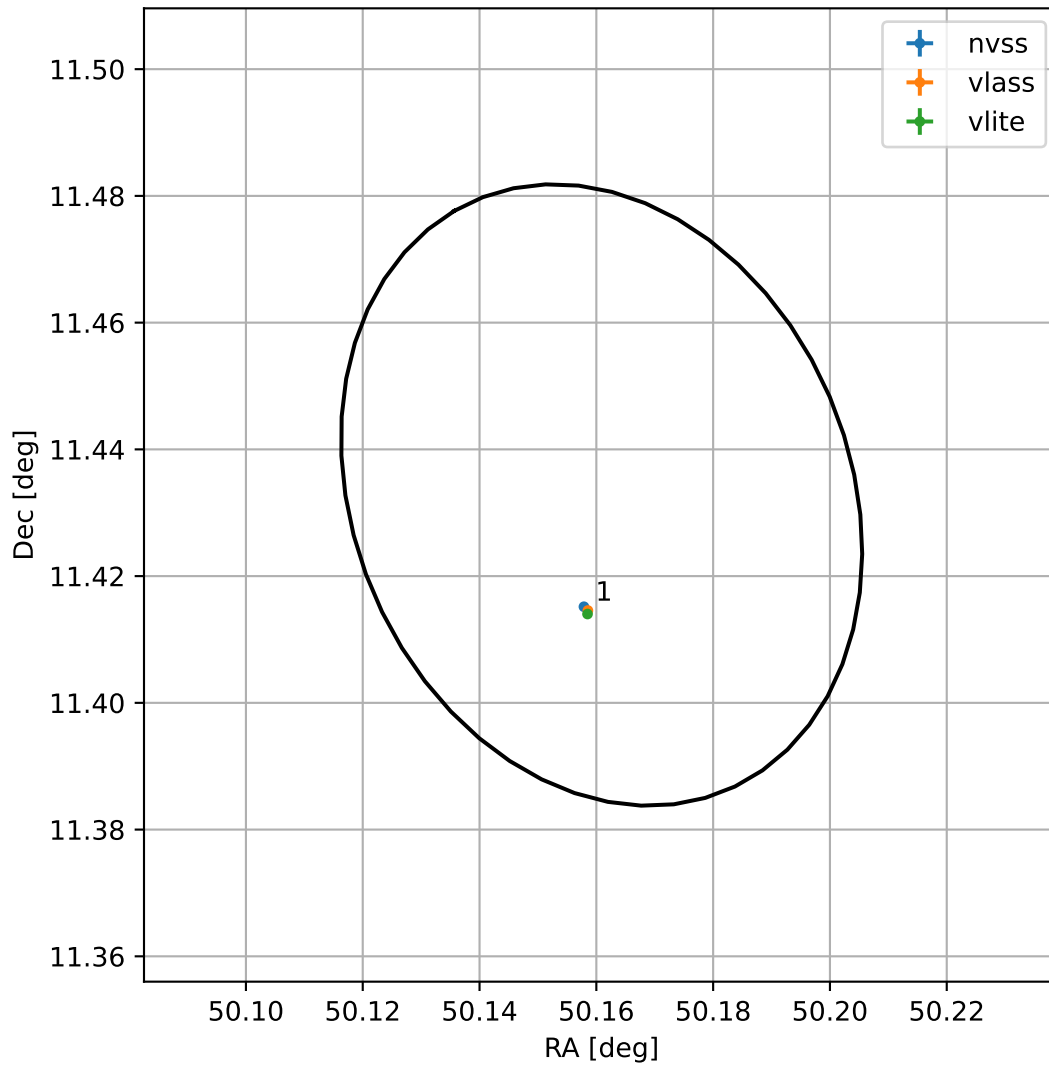
4FGL J0320.6+1125
