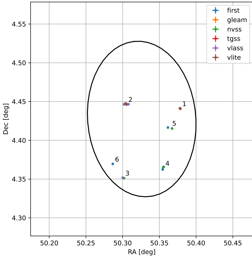
4FGL J0321.3+0425
