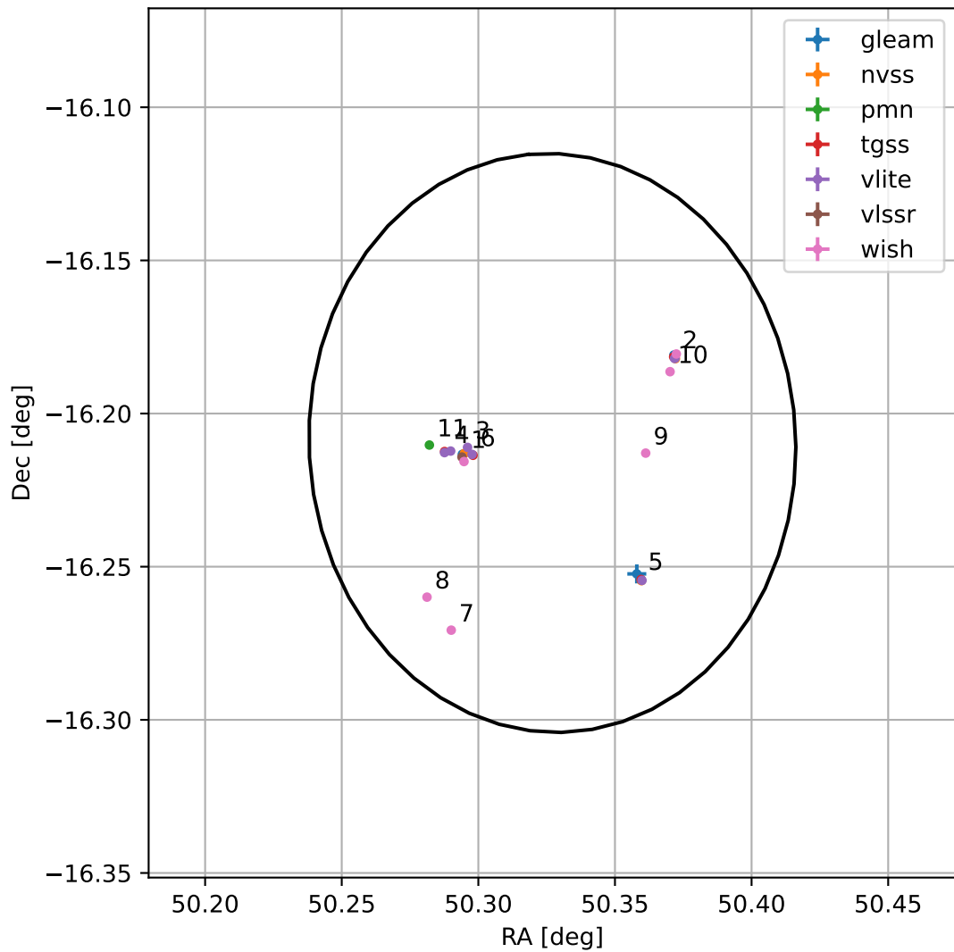
4FGL J0321.3-1612
