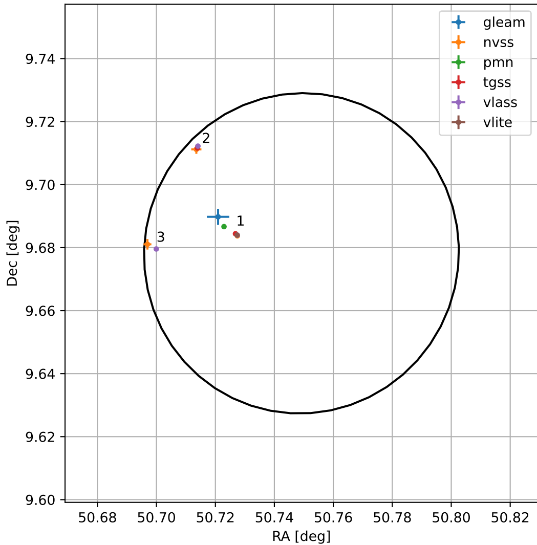
4FGL J0322.9+0940
