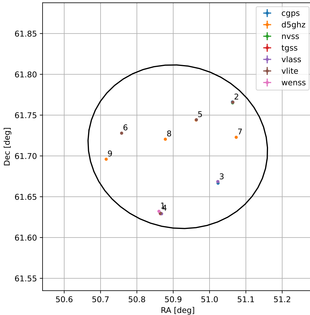
4FGL J0323.6+6142
