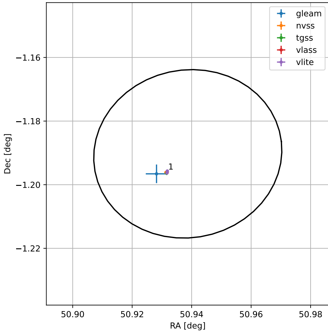
4FGL J0323.7-0111
