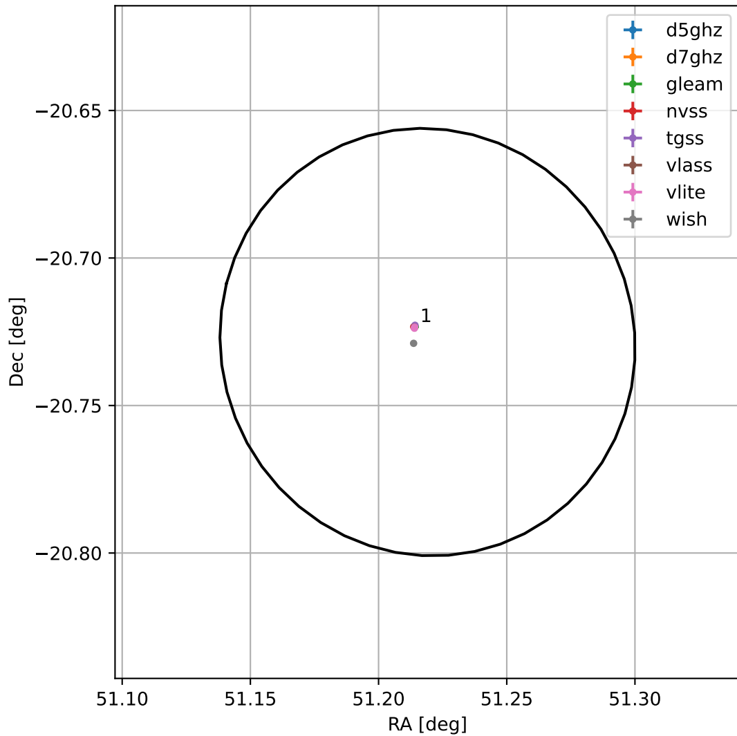
4FGL J0324.8-2043
