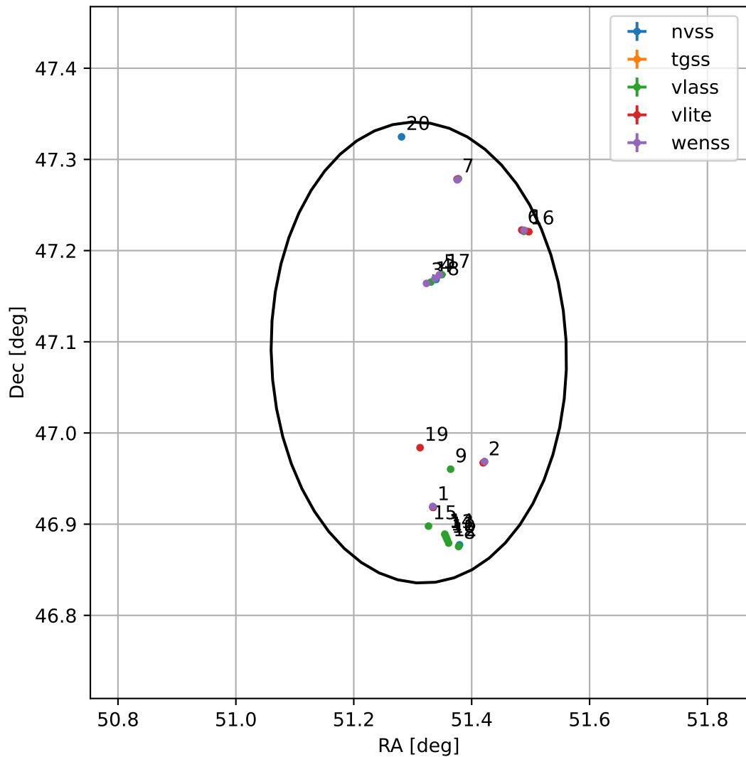
4FGL J0325.2+4705
