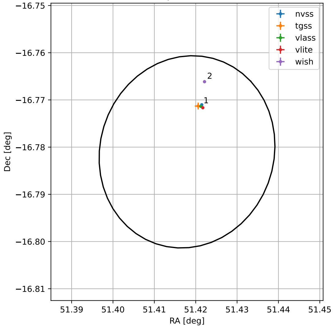
4FGL J0325.6-1646
