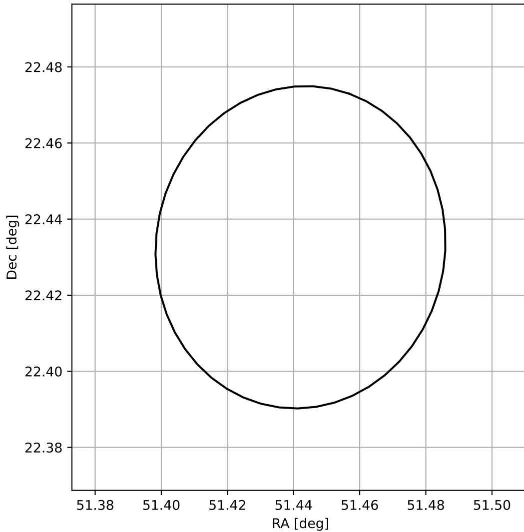
4FGL J0325.7+2225
