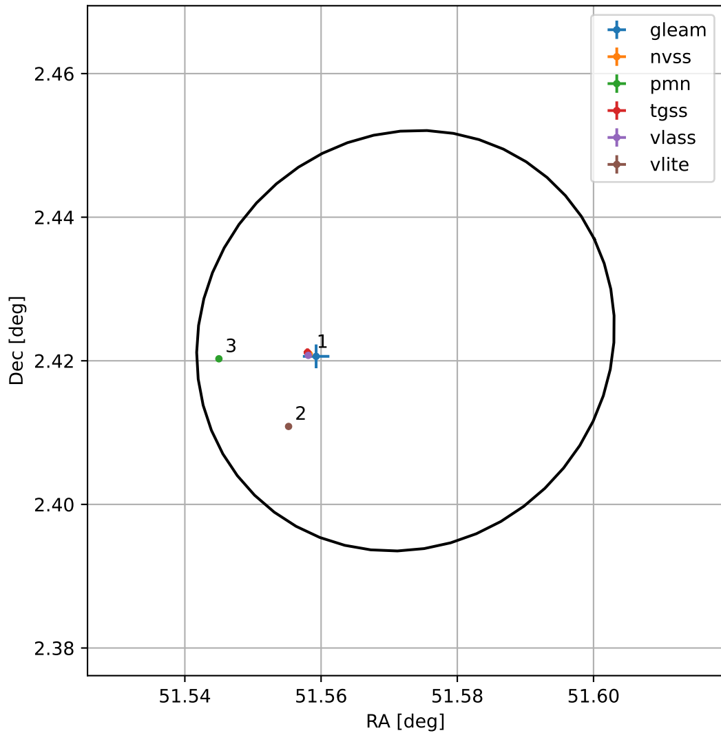
4FGL J0326.2+0225
