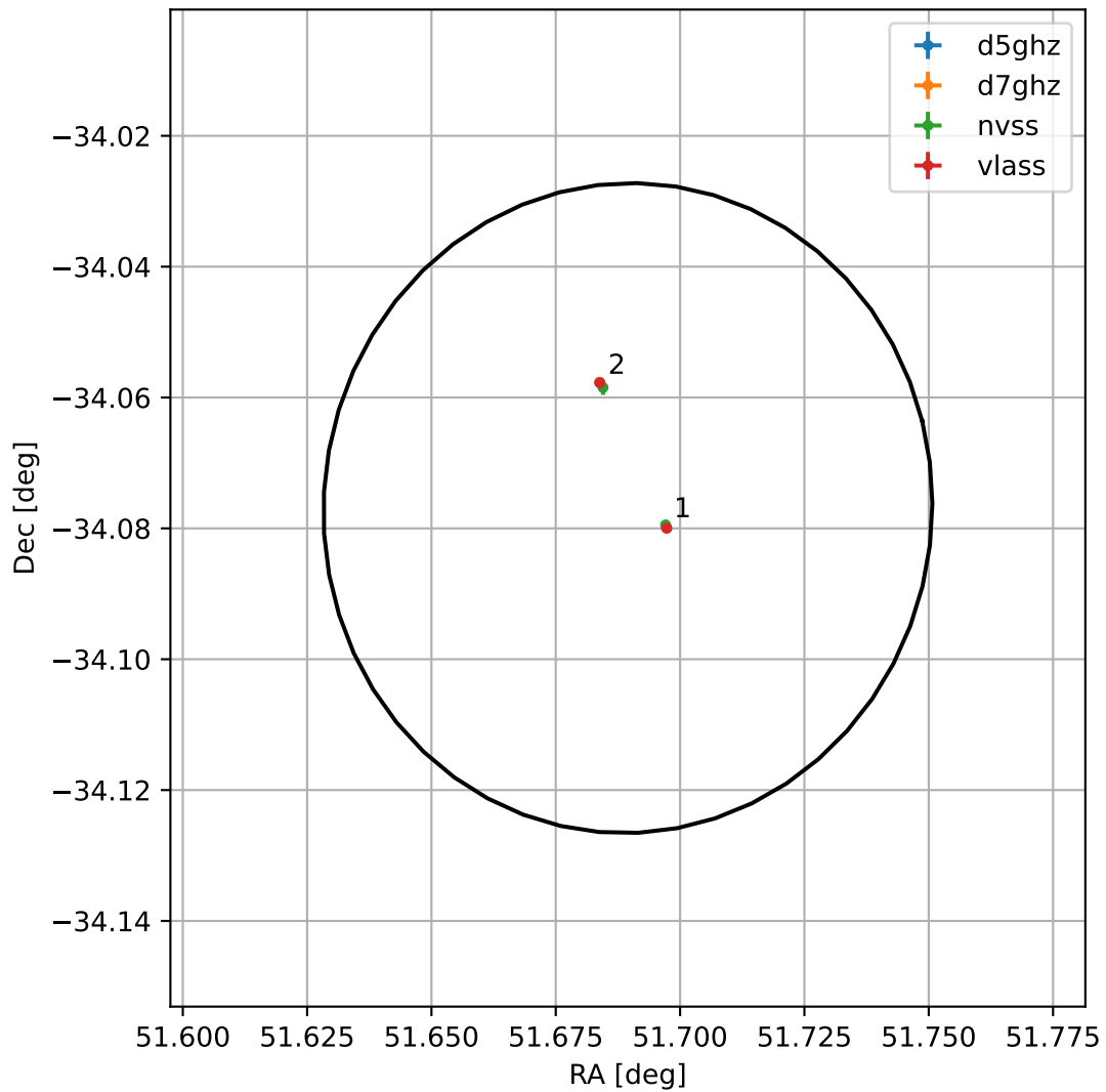
4FGL J0326.7-3404
