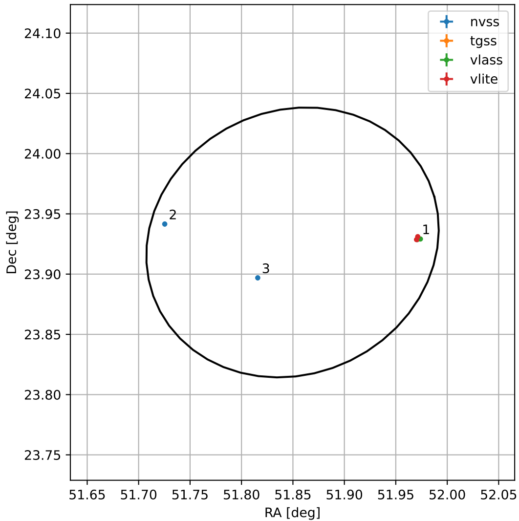
4FGL J0327.3+2355
