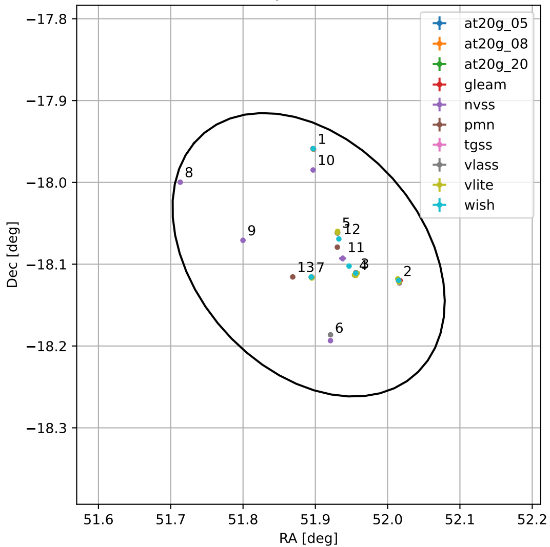
4FGL J0327.5-1805
