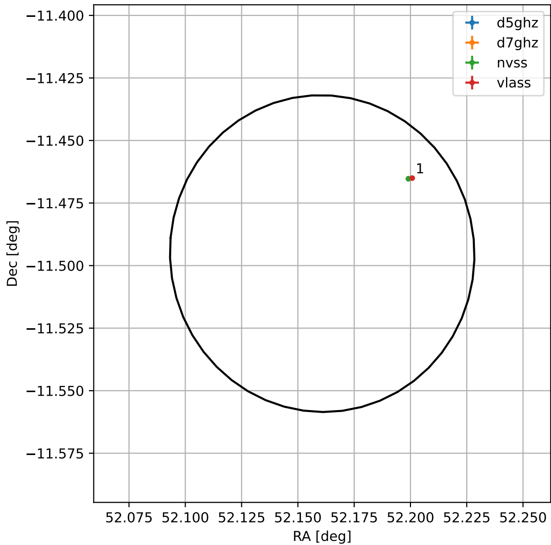
4FGL J0328.6-1129
