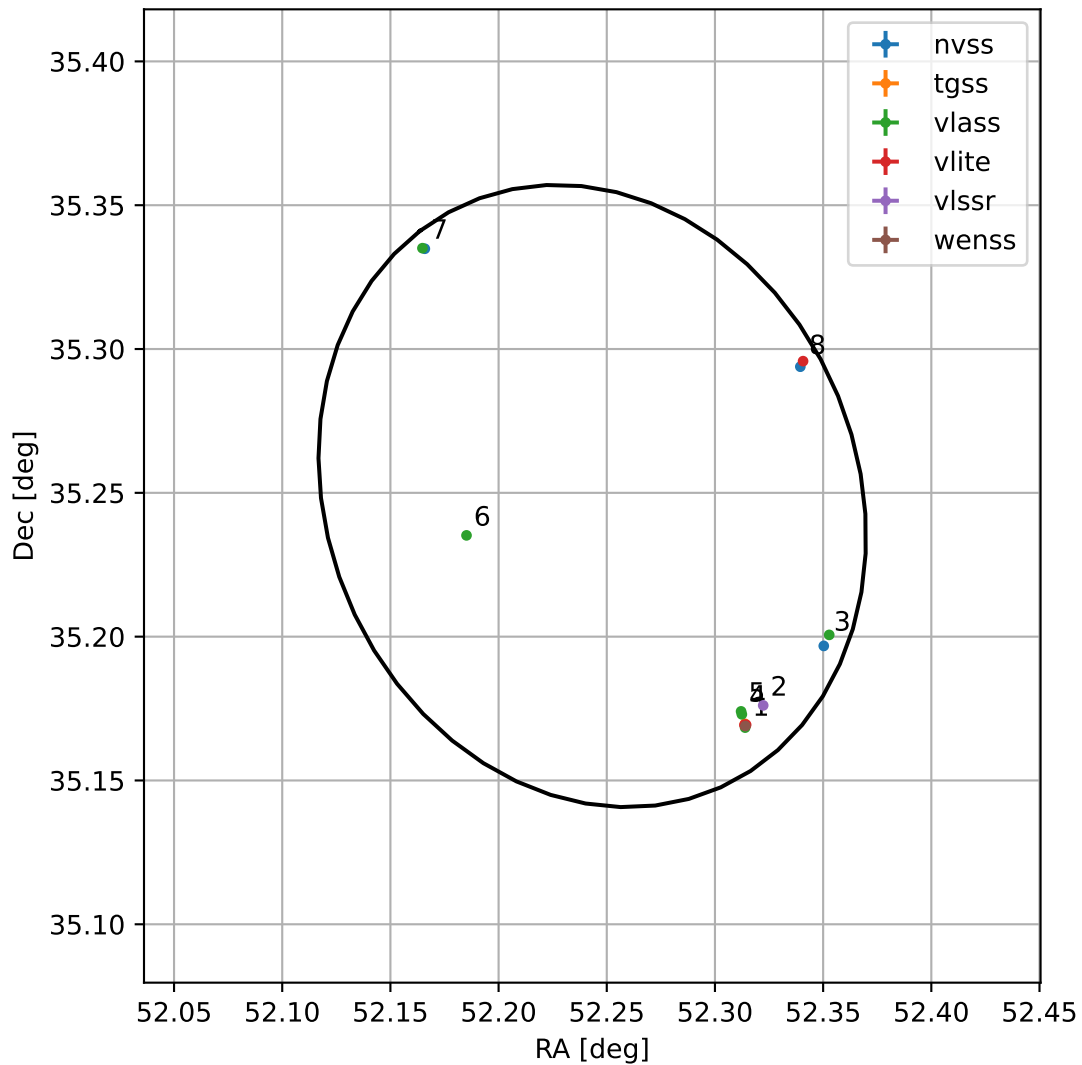
4FGL J0328.9+3514
