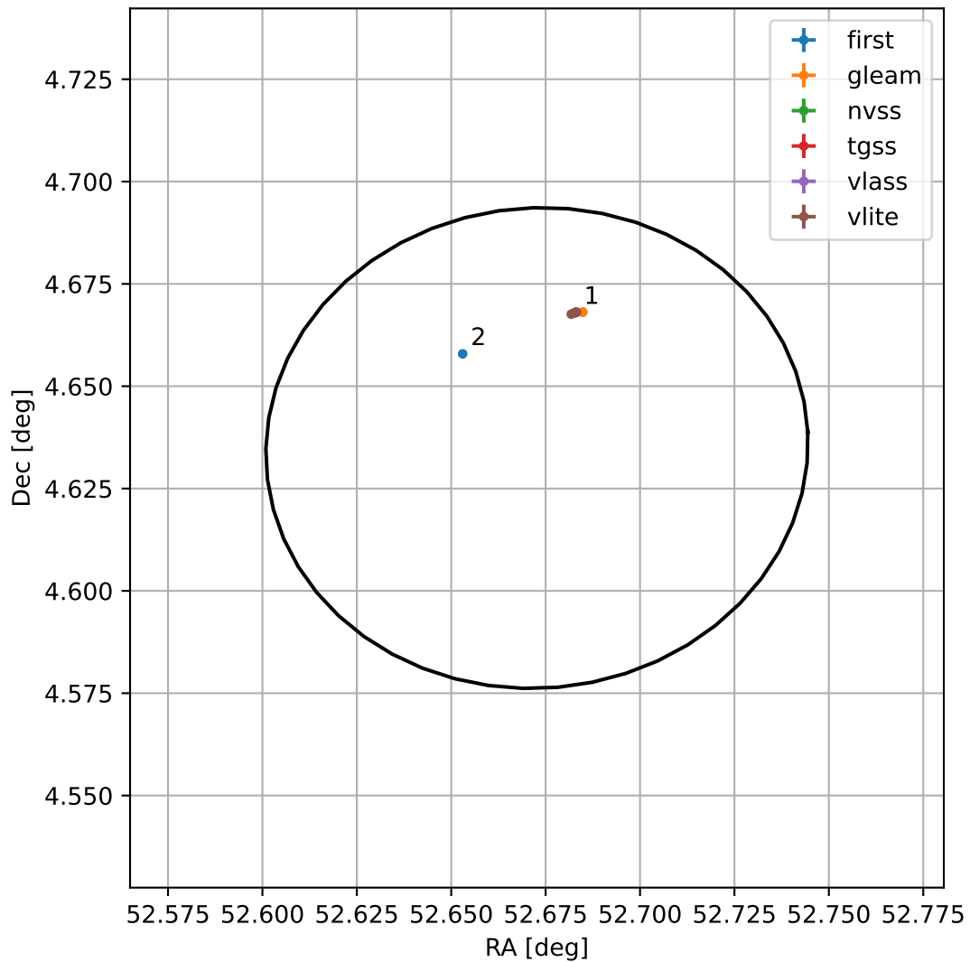
4FGL J0330.6+0438
