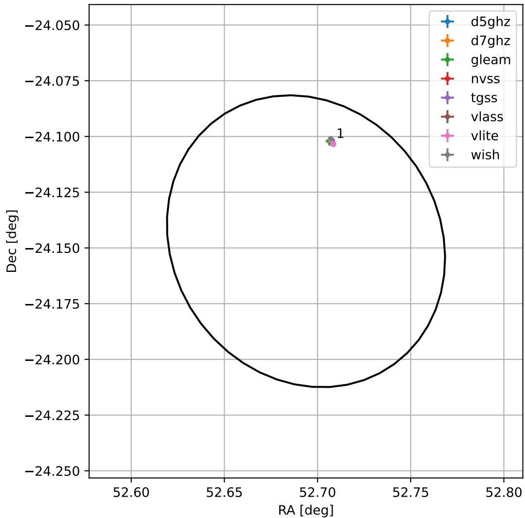
4FGL J0330.7-2408
