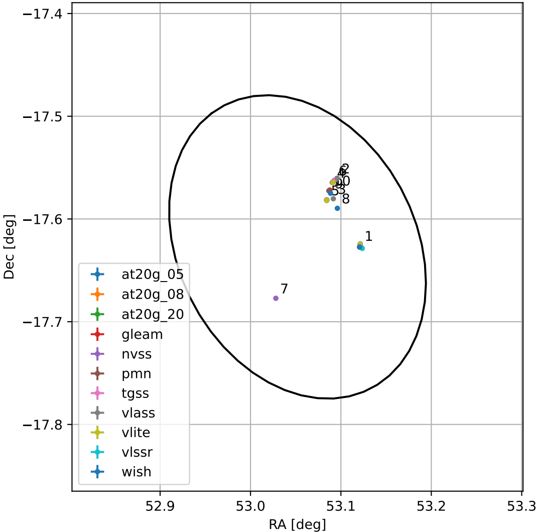
4FGL J0332.2-1737
