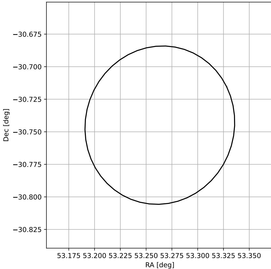
4FGL J0333.0-3044
