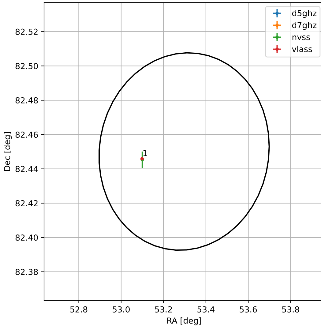
4FGL J0333.1+8227
