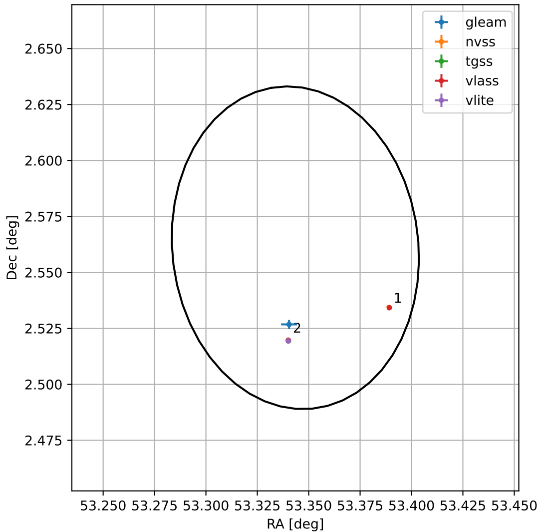
4FGL J0333.3+0233
