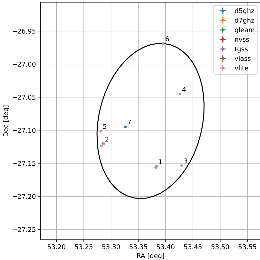
4FGL J0333.4-2705
