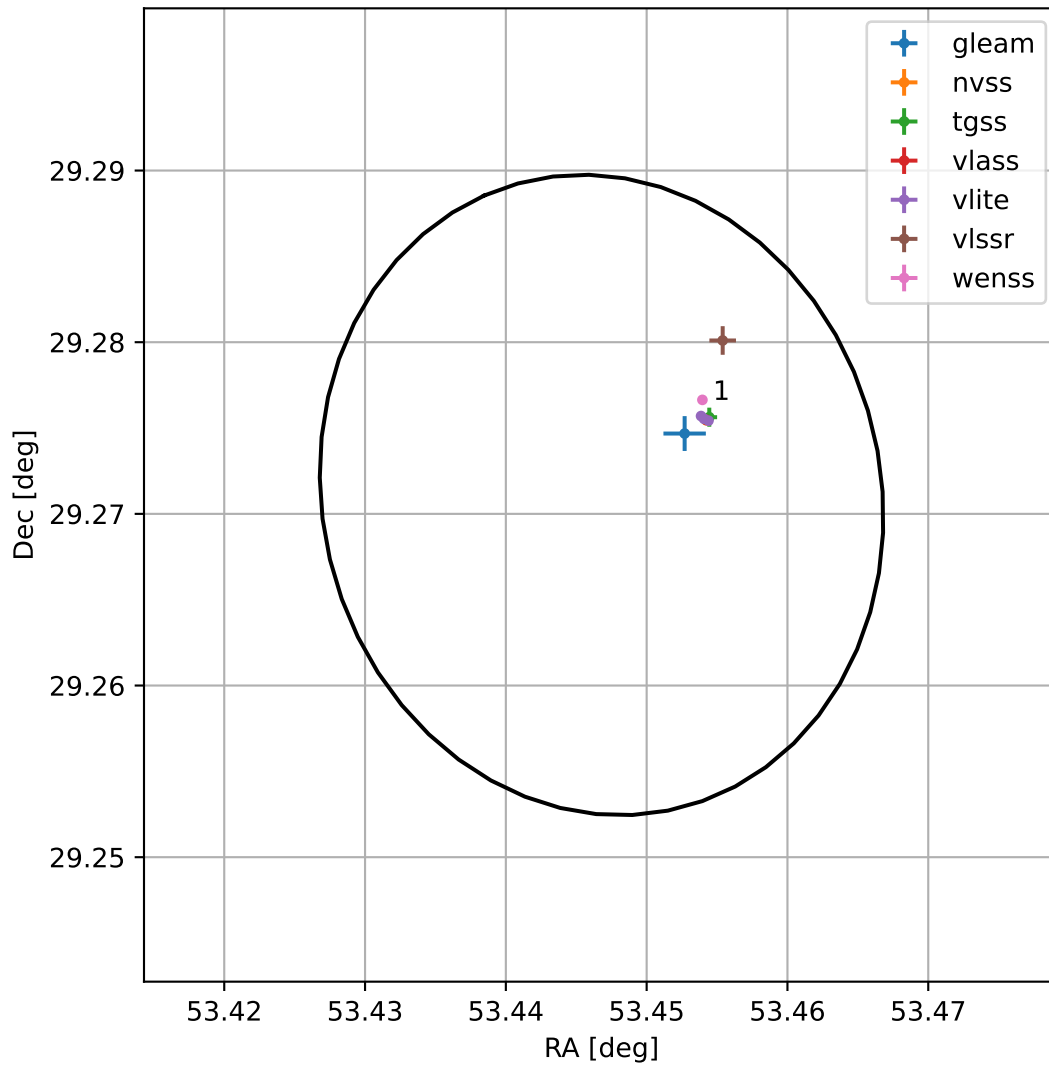
4FGL J0333.7+2916
