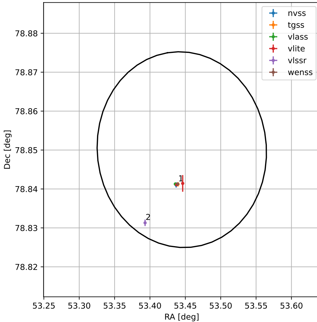
4FGL J0333.7+7851
