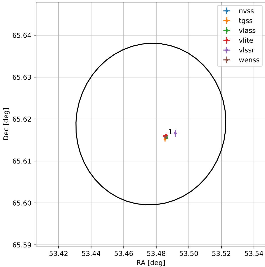
4FGL J0333.9+6537
