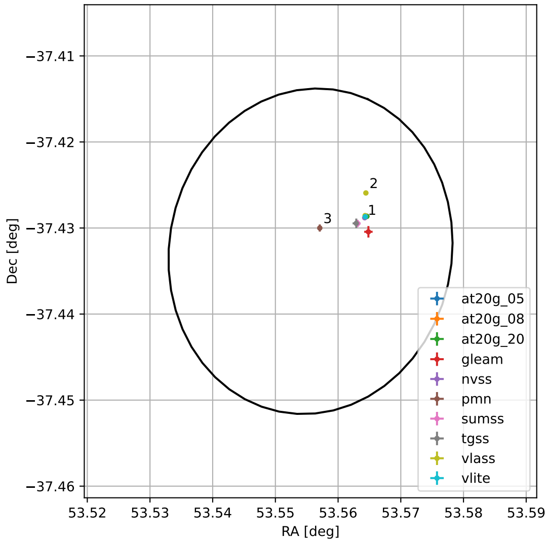
4FGL J0334.2-3725
